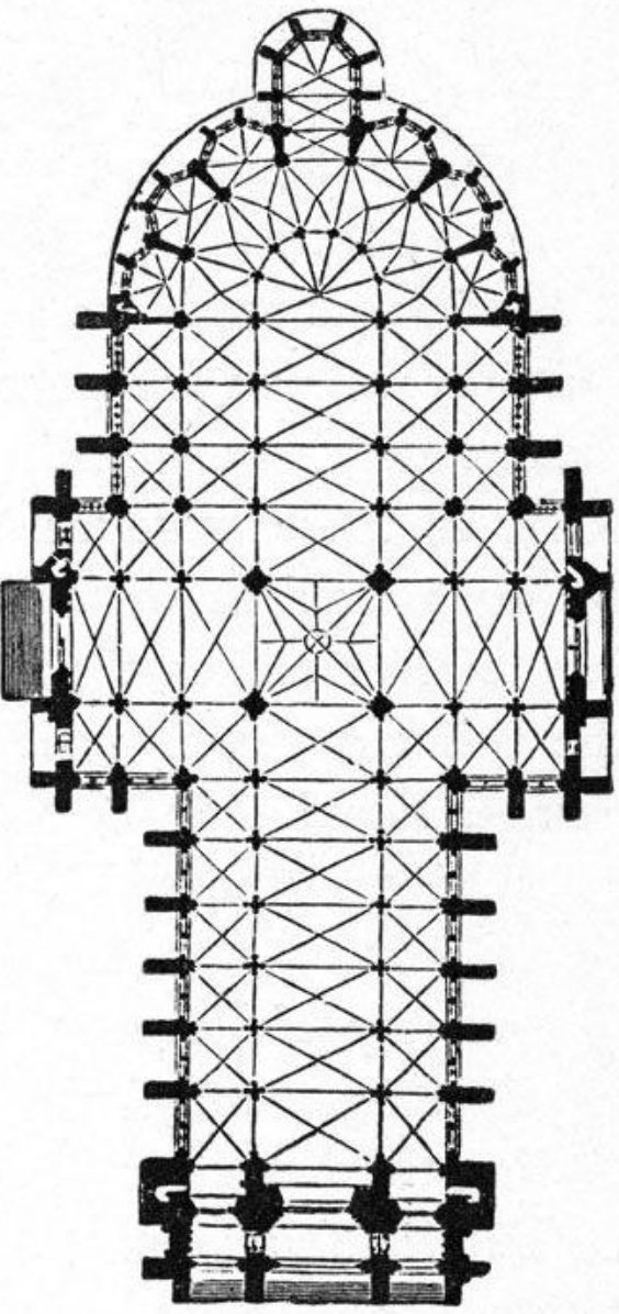
Fig. 291. Ground-Plan of the Cathedral of Amiens.
