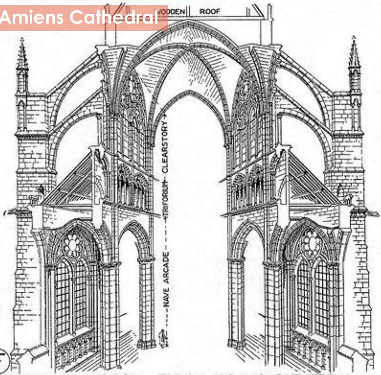
TRANSVERSE SECTION OF A TYPICAL GOTHIC CATHEDRAL (AMIENS)
